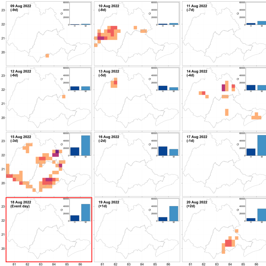
Daily Rainfall RP and Discharges at MRB: 2022-08-18
