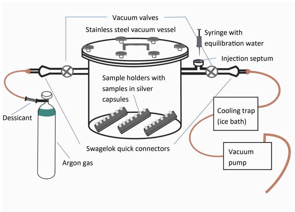
Fig: Schematic diagram of steam equilibration device
