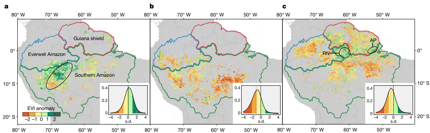
Fig. 1 | Amazon forest remotely sensed responses to droughts. a–c , Amazon forest remotely sensed responses to the droughts of 2005 ( a ), 2010 ( b ) and 2015/2016 ( c ), expressed as standardized anomalies of multiangle implementation of atmospheric correction (MAIAC) EVI (a proxy of photosynthetic capacity) in drought-affected pixels (defined in Extended Data Fig. 1a–c). Note that a highlights an ellipse of green-up and brown-down patterns that correspond to shallow and deep water tables in Fig. 2a; c highlights two areas exhibiting green-up—RN, in the Rio Negro catchment and AP in Amapá state—for comparison to Figs. 4 and 5. Insets show the frequency
