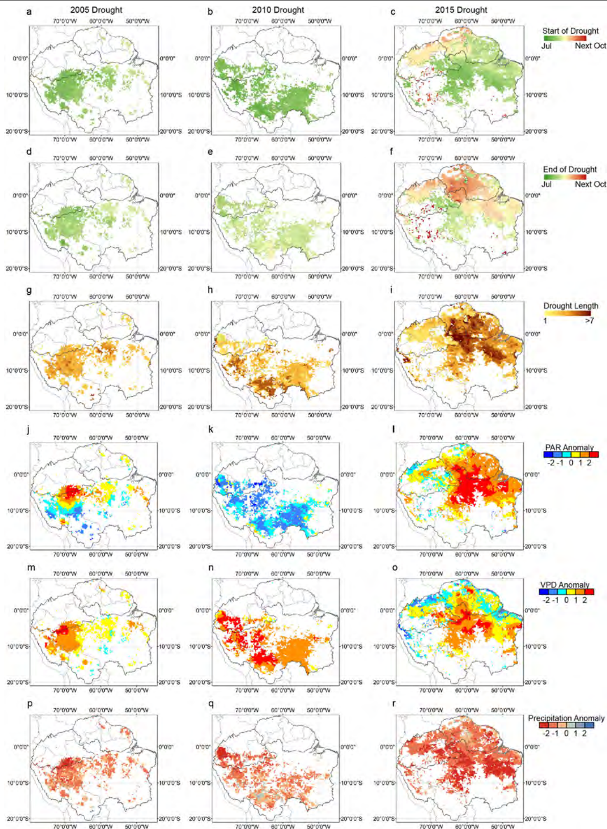
Extended Data Fig. 3 | Spatial distributions of climate dynamics in the 2005, 2010 and 2015 droughts. a–i, Spatial distributions of climate dynamics in the 2005 (left column), 2010 (middle column) and 2015 (right column) droughts for: (a)–(i): Drought dynamics showing drought onset date (row 1, a–c), drought end date (row 2, d–f), and drought duration (row 3, g–i, end date minus start date). Pixel-by-pixel drought responses (EVI in Figs. 1–4; or GOSIF in Extended
