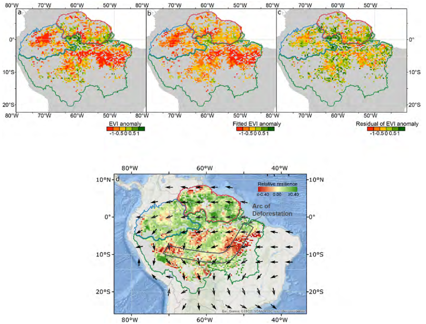
Extended Data Fig. 10 | Modeled forest response to the 2015 drought and implications of the derived map of Amazon forest biogeography. a–c, Forest response to the 2015 drought in drought-affected pixels. (a) Observed EVI anomalies (resampled at 0.4 degrees to match model resolution which accounts for spatial autocorrelation (see Supplementary Fig. 1)). (b) GAM-predicted EVI anomalies (model of Supplementary Table 1d). (c) Residual EVI anomalies (panel a observations minus panel b predictions). The GAM well-predicts the pattern of response (Panel b), but under-estimates the extremes of the responses (as evident from residuals in panel c continuing to show
