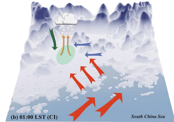
convection initiation mechanisms
