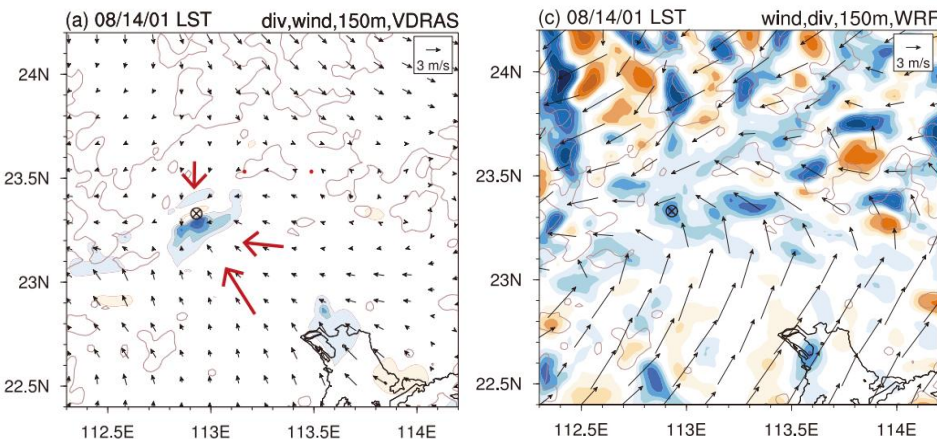
horizontal winds and divergence
