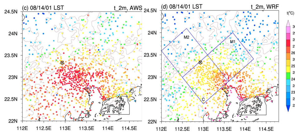
2-m temperature
