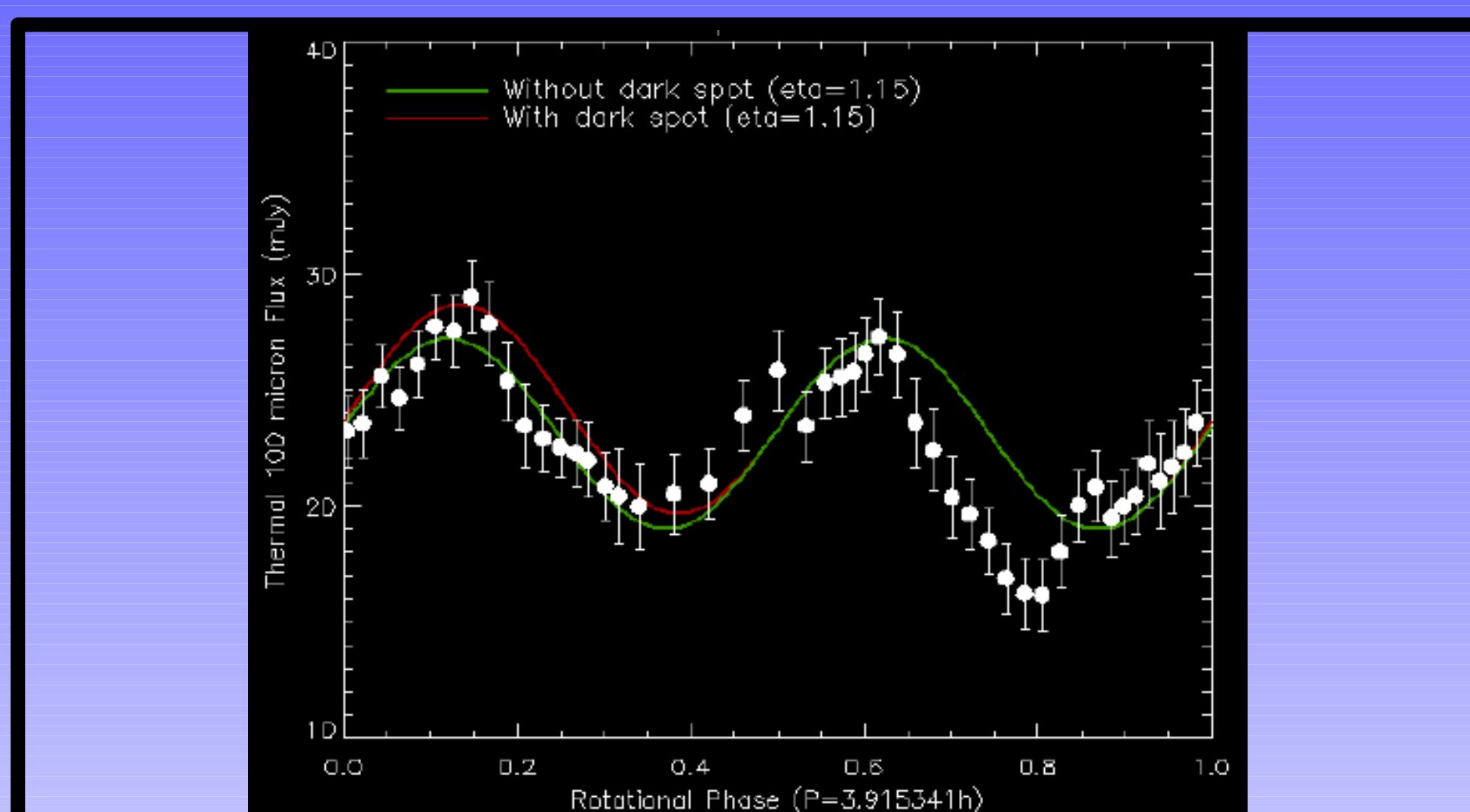
Fig. 3. Haumea lightcurve observed twice with PACS 100 \mu m channel and a modeled LC [12] with and without a dark spot (shape model 2 in P II). The thermal and visible lightcurves are correlated (shape effect) with a factor of variation 2 in thermal and 1.3 in visible. We find no clear evidence of a dark spot. Thermal inertia is very low and the surface is porous.
