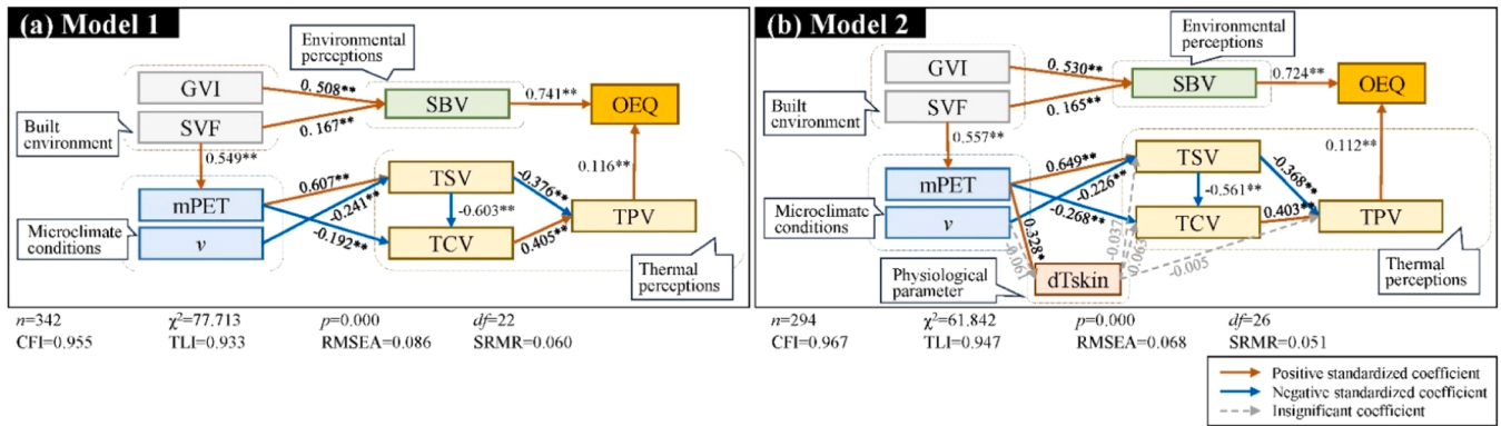
Fig. 5. Pathway models (a) among built environment characteristics, microclimate conditions, and thermal and multisensory perceptions, (b) with physiological parameter included. ( Note: df degree of freedom, CFI Comparative Fit Index, TLI Tucker-Lewis Index, RMSEA Root Mean Square Error of Approximation, SRMR Standardized Root Mean Square Residual.).
