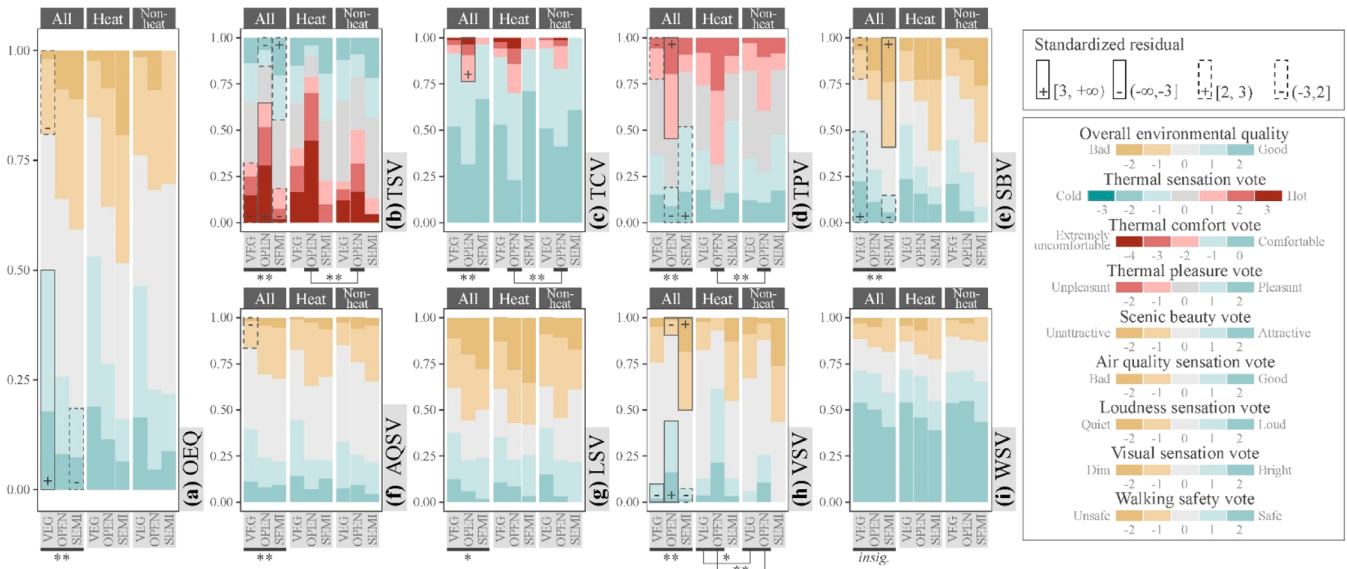
Fig. 3. Percentage of thermal and environmental perception votes in different types of public spaces under extreme-heat, non-extreme-heat, and both conditions ( n_{\text{All}}=342 , n_{\text{Heat}}=186 , n_{\text{Non-heat}}=156 ). (Note: * and ** refer to significance at 0.05 (two-tailed) and 0.01 (two-tailed) respectively. Same below. Pearson standardized residual quantifies the contribution of each category to the overall chi-square statistic, and the contribution can be seen as evident when greater than 2, the more evident, the greater.).
