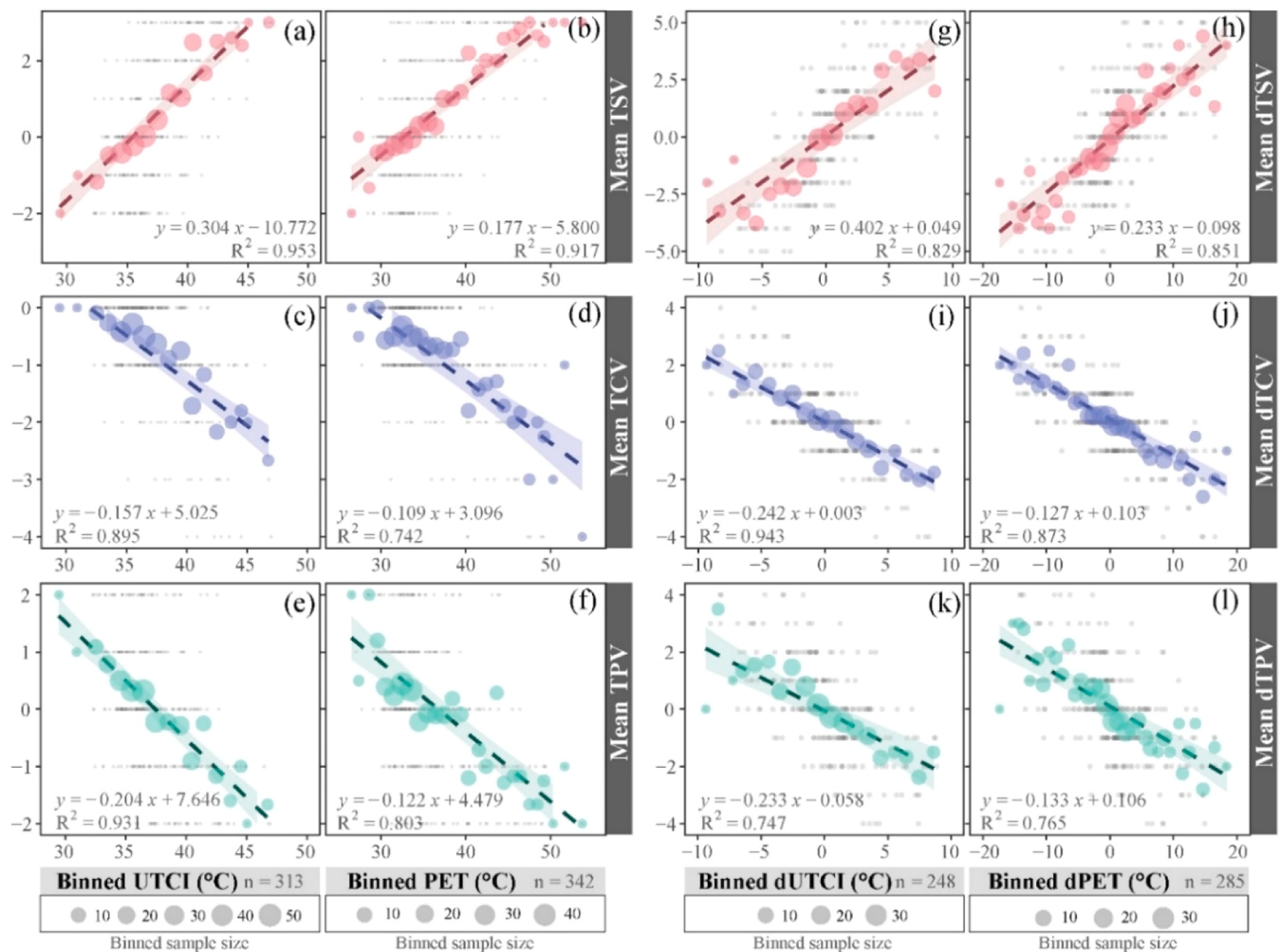
Fig. 6. Linear regression models between binned UTCI, PET and (a-f) mean thermal perception votes, (g-l) mean difference of thermal perception votes between two adjacent stopping points. ( Note: Legend shows the binned sample size. Shaded areas refer to 95 % confidence interval.).
