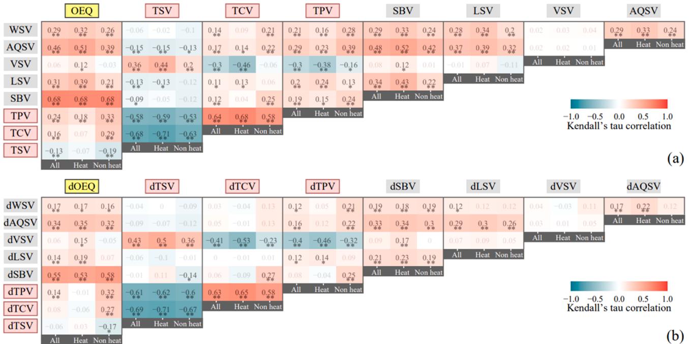
Fig. 4. Kendall's tau correlation coefficients among thermal and environmental perceptions under extreme-heat and non-extreme-heat conditions with (a) data at all stopping points ( n_{\text{All}}=342 , n_{\text{Heat}}=186 , n_{\text{Non-heat}}=156 ), and (b) differences between two adjacent stops ( n_{\text{All}}=285 , n_{\text{Heat}}=155 , n_{\text{Non-heat}}=130 ).
